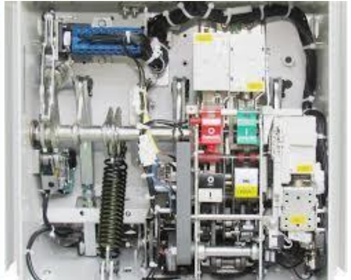
VD4 Medium Voltage VCB
